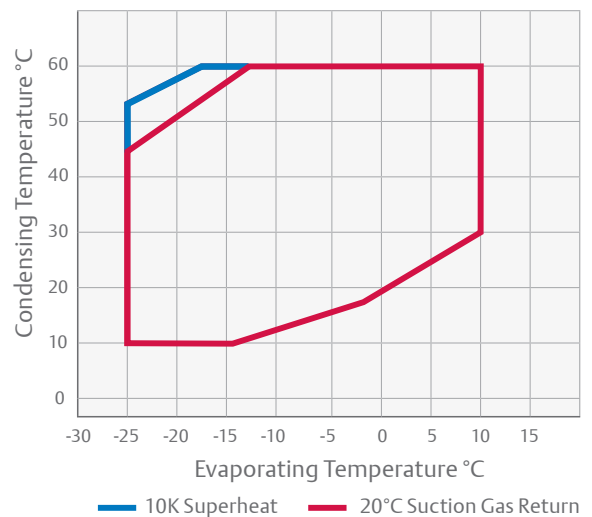
YBD - R455A
