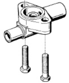
Straight Through Flange (DL)
