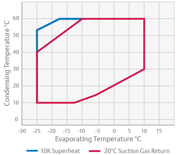
YBD - R454A
