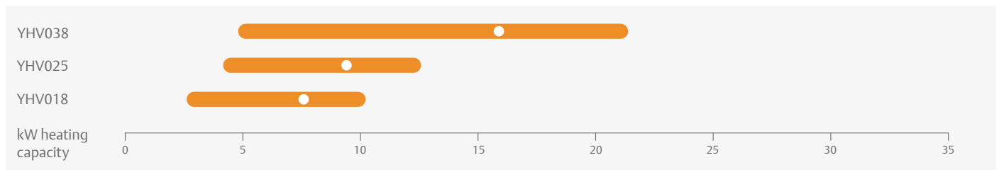
YHV Copeland scroll variable speed compressor and drive
