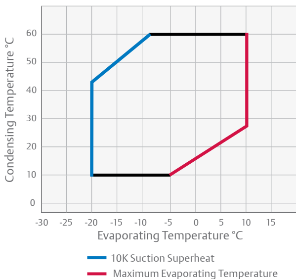
YB - R1234yf
